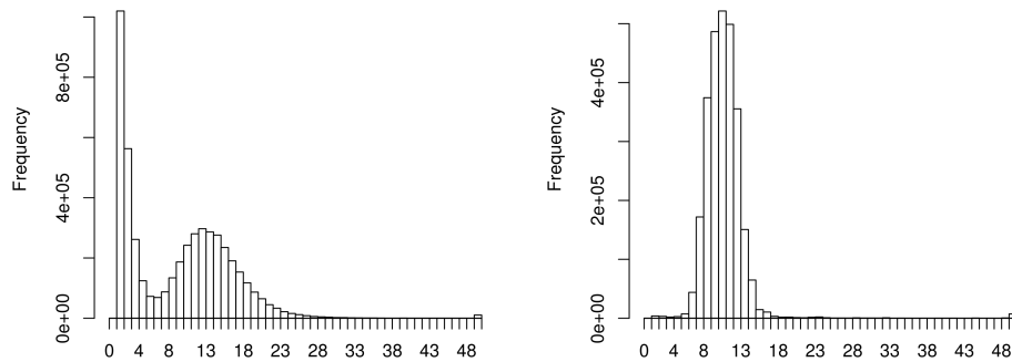
Figure 10: Weighted k-mer coverage histograms of the paired-end reads pre-trimmed (left) and post-trimmed (right).
